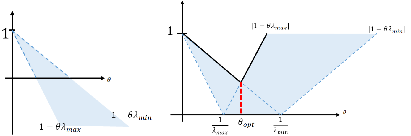
Figure 21.32: Finding the optimal \theta for Richardson iteration.
