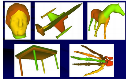
Shape Segmentation
