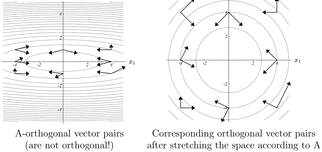
Figure 9.24: Visualization of the concept of A-orthogonality.
