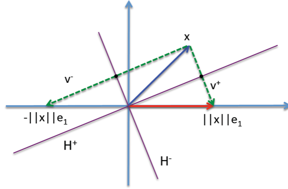
Figure 12.28: The two alternative Householder reflections.
