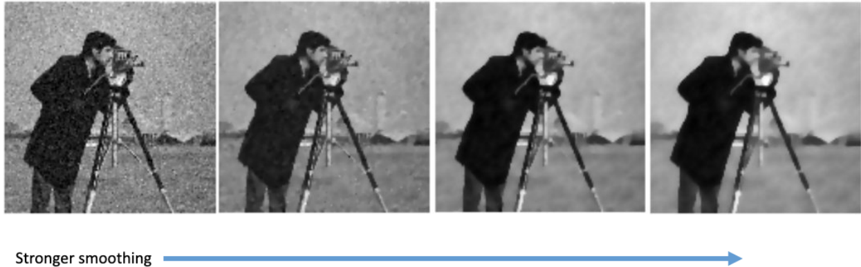
Figure 7.19: Effect of increasing the regularization parameter \alpha with total variation regularization.
