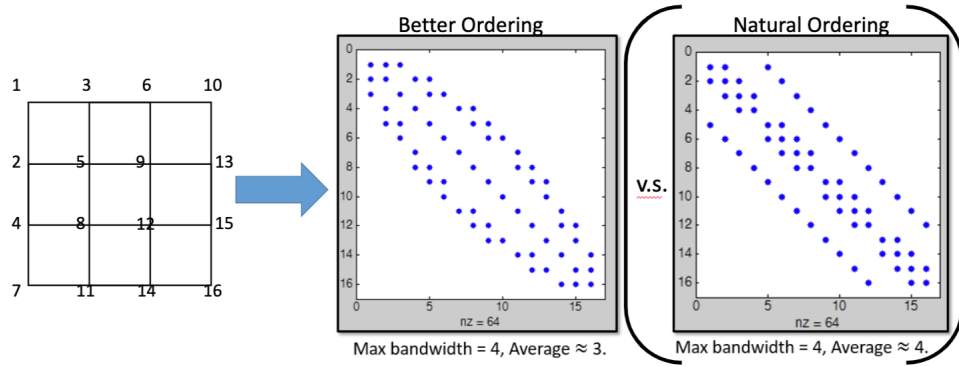
Figure 6.8: Level sets of an example graph.
