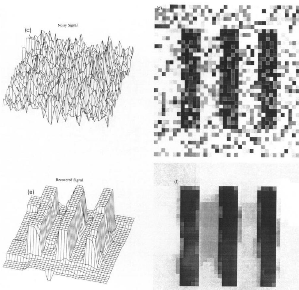
Figure 7.17: Noisy image (top) and denoised image (bottom) using total variation regularization [Rudin et al. 1992].
