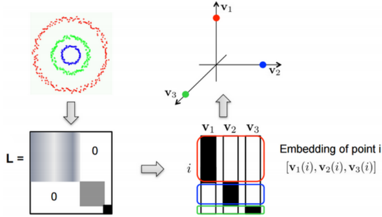
Figure 17.30: Steps of spectral clustering.
