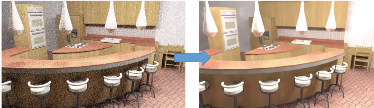
Figure 7.14: Example noisy synthetic image (left) and denoised image (right) from [Kalantari et al. SIGGRAPH 2015].
