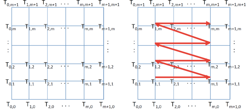
Figure 4.4: Two-dimensional indexing (left) for a discrete plate and a possible 1D ordering/flattening (right).
