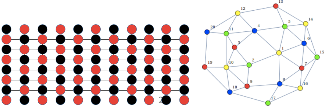
Figure 8.21: Example colorings for parallelizing the Gauss-Seidel iteration.
