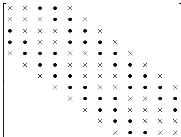
Figure 6.7: Example of where fill can occur for banded matrices. The possible fill occurs where \bullet are depicted.
