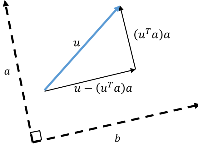
Figure 9.25: Orthogonalizing a vector u with respect to a .
