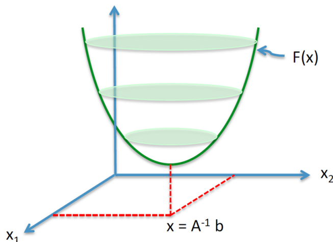
Figure 9.22: Visualization of F(x) when n = 2 .
