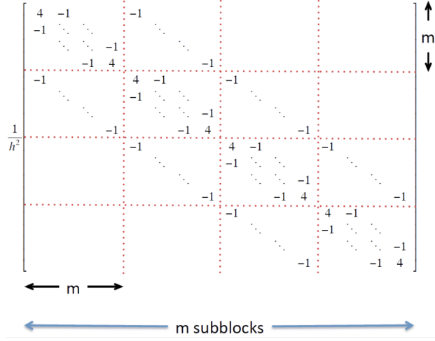
Figure 4.5: General matrix structure for discrete Laplacian with natural rowwise ordering.
