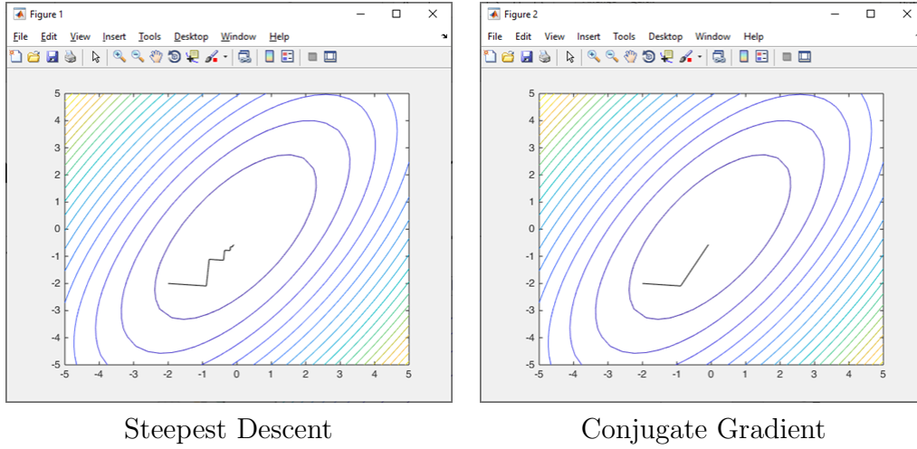
Figure 9.26: Comparison of steepest descent and conjugate gradient methods in \mathbb{R}^2 .
