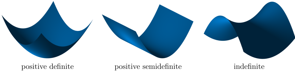
Figure 2.1: Plotting of f = x^T A x as a height function with x \in \mathbb{R}^2 and different A \in \mathbb{R}^{2 \times 2} .
