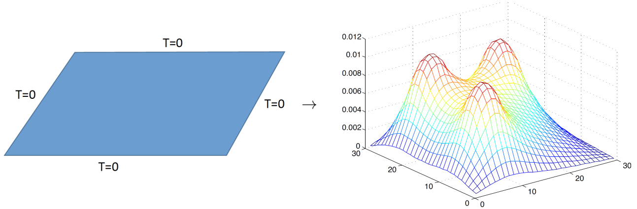
Figure 4.2: Two-dimensional plate domain (left) and heat distribution (right).
