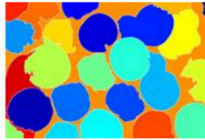
Image Segmentation
