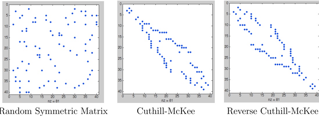
Figure 6.9: Comparison of CM (middle) vs RCM (right) for a symmetric matrix (left).
