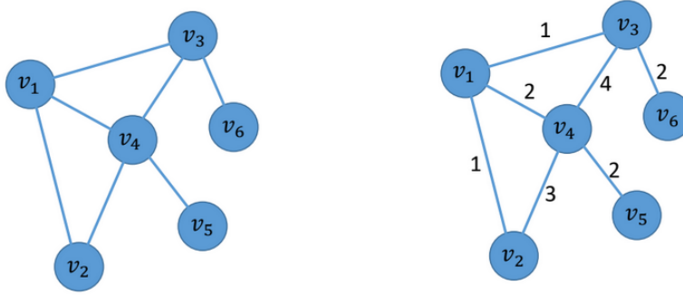
Figure 17.29: Example graph G(V, E) (left) and the same graph with weighted edges (right).
