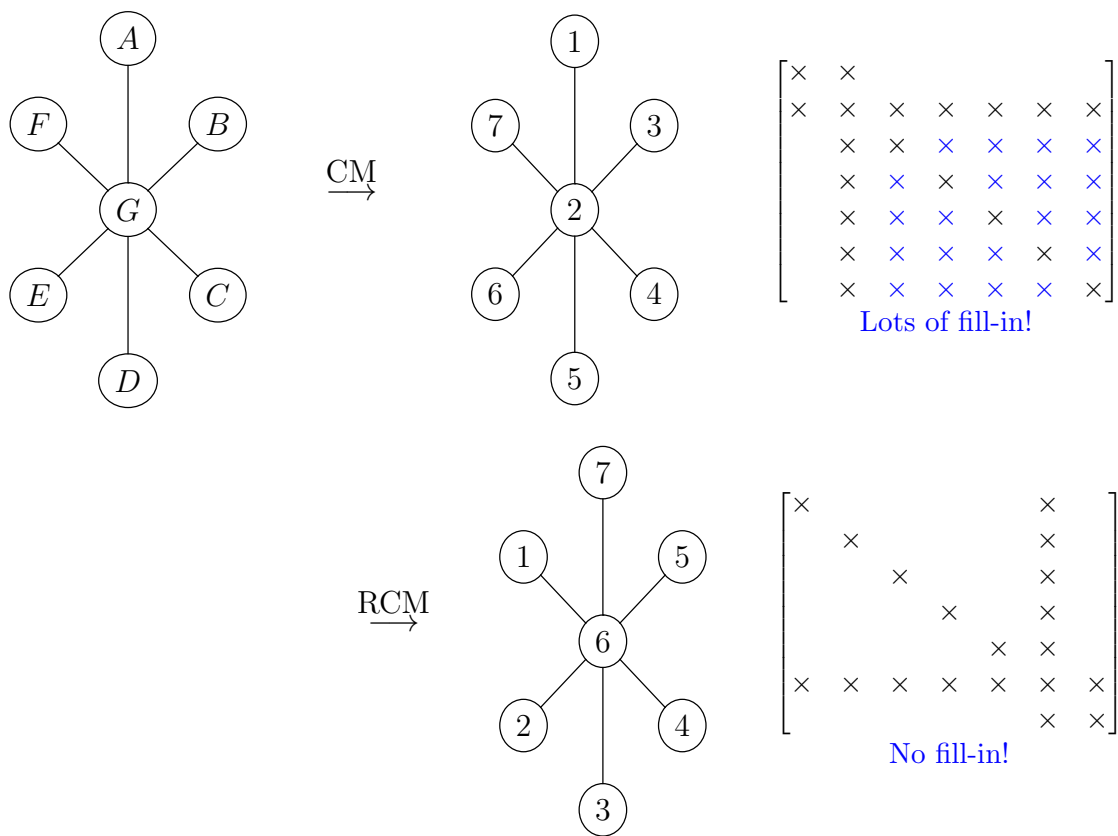
Figure 6.10: CM and RCM orderings for the initial graph (top left). The CM algorithm is started at node A and ties are broken alphabetically.
