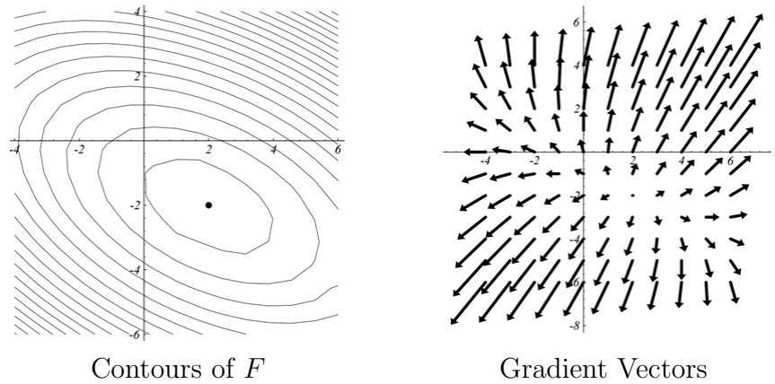
Figure 9.23: Example contours and gradient vectors of a function F .
