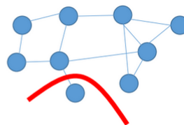
Computed cut
