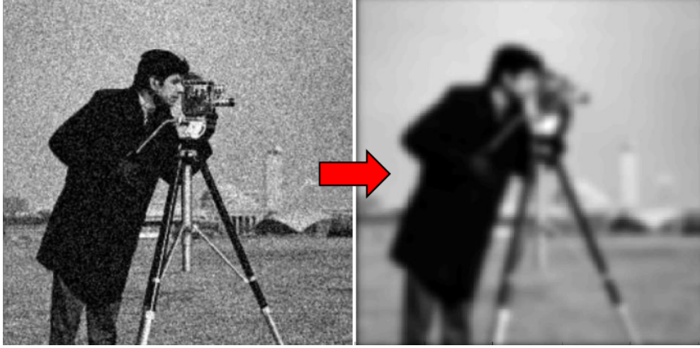
Figure 7.16: Laplacian regularization for image denoising of the noisy image (left). The result on the right is smeared out throughout the image.
