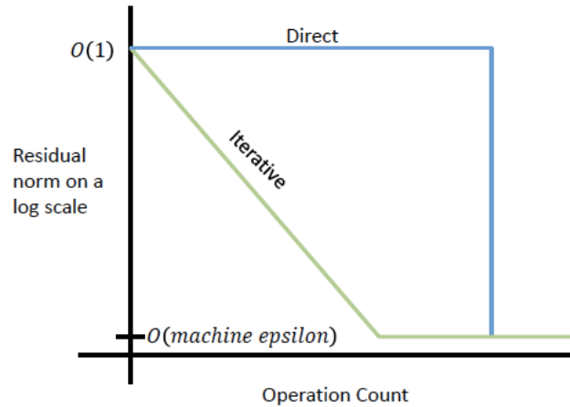
Figure 8.20: Comparison of the path to solutions of iterative versus direct methods.
