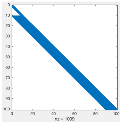
Cholesky Factor
