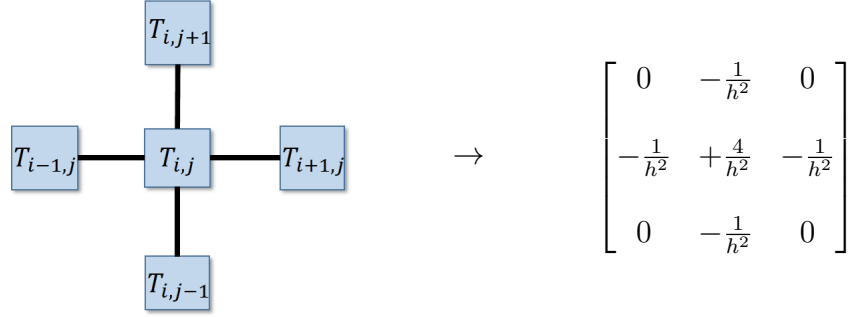
Figure 4.3: The finite difference stencil for the left hand side of (4.10), i.e., the negative of the 2D discrete Laplacian.
