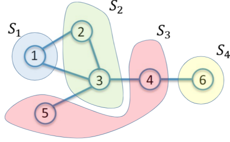
Figure 6.8: Level sets of an example graph.
