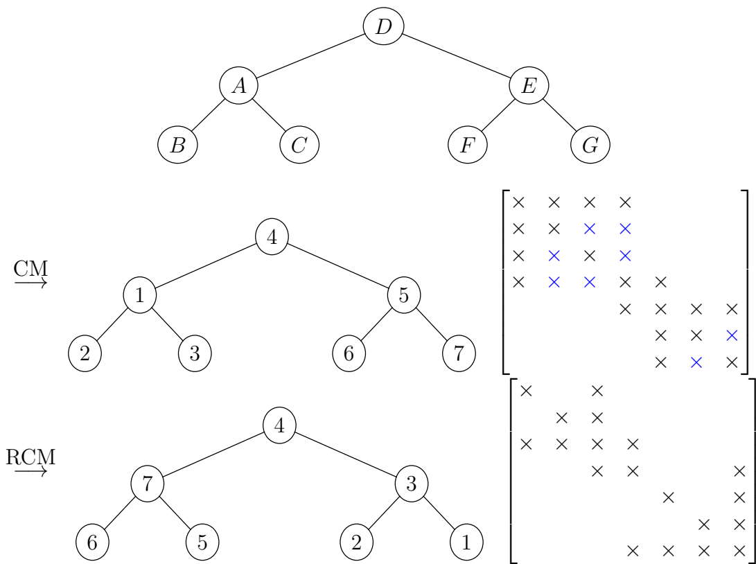
Figure 6.11: CM and RCM ordering for a tree graph. Notice that RCM produces a reordering with no fill (shown as \times ).
