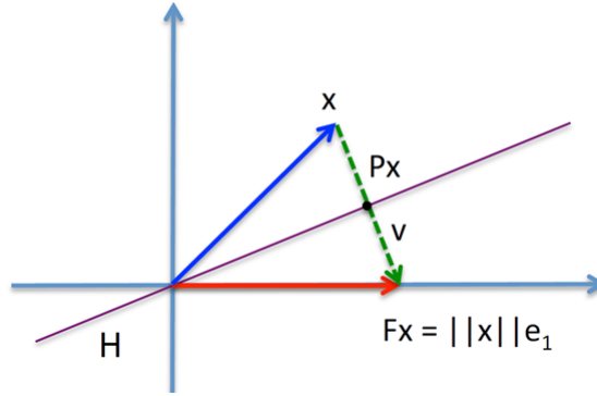
Figure 12.27: Applying the Householder reflector F to the vector x , which reflects x across the hyperplane H .
