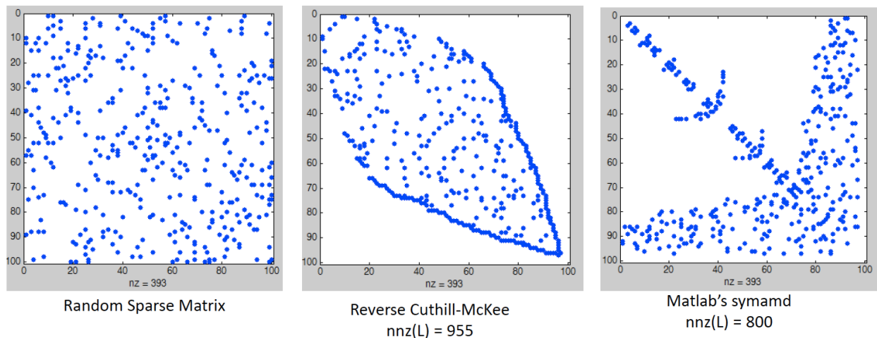
Figure 7.12: Comparison of reordering techniques RCM and AMD for a random sparse matrix.
