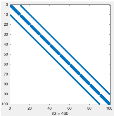
Laplacian A
