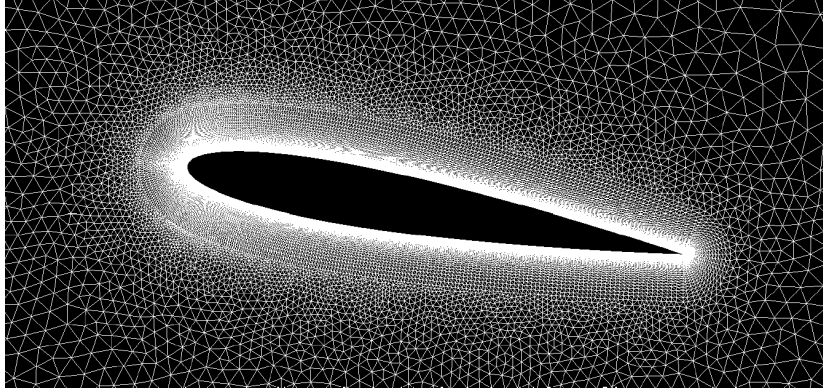
Figure 4.6: Example discretization using triangles for an airfoil.
