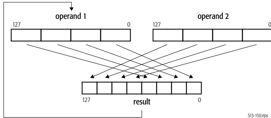
Figure 4-4. Pack Operation
