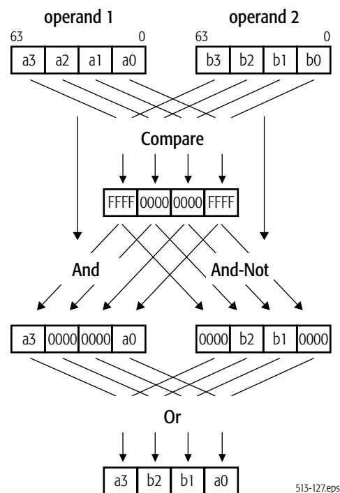
Figure 5-5. Branch-Removal Sequence
