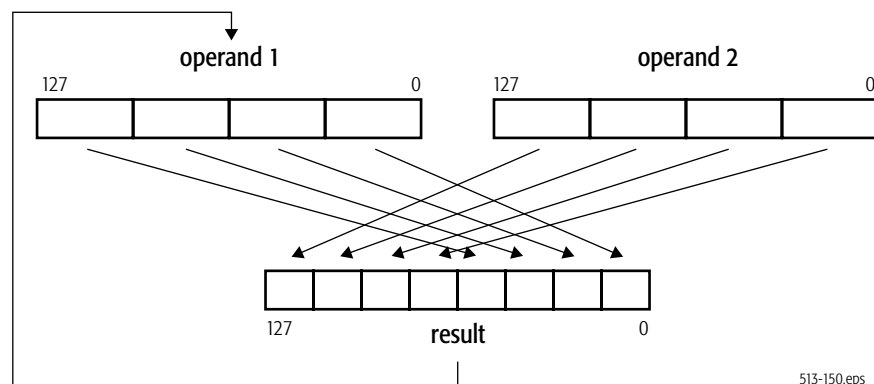
Figure 4-20. PACKSSDW Pack Operation
