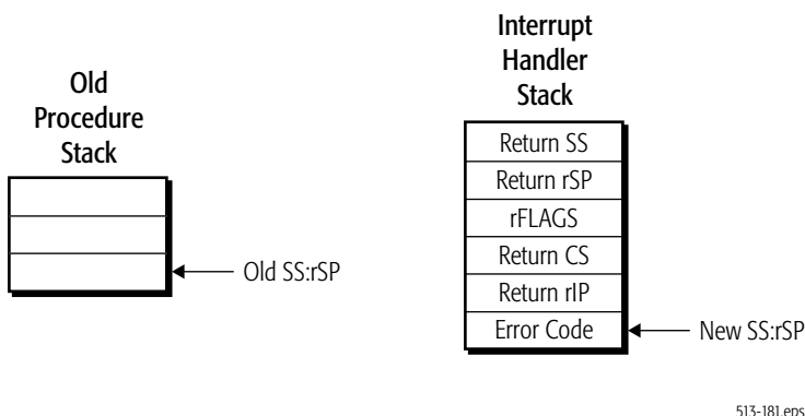
Figure 3-17. Procedure Stack, Interrupt to Higher Privilege
