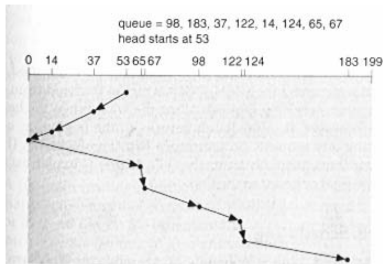
Figure 14.3 SCAN disk scheduling.
