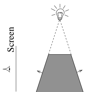
Shadow Volume
