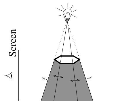
Multiple Polygons
