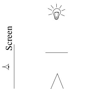
Scene
