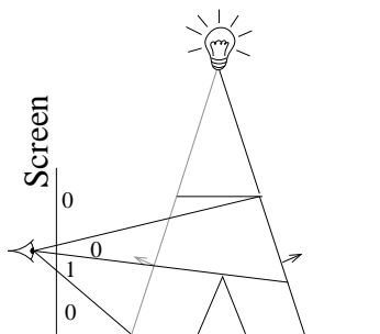
Back facing -1
