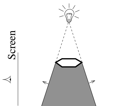
Silhouette
