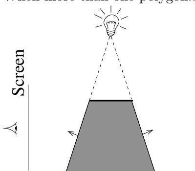
Single Polygon
