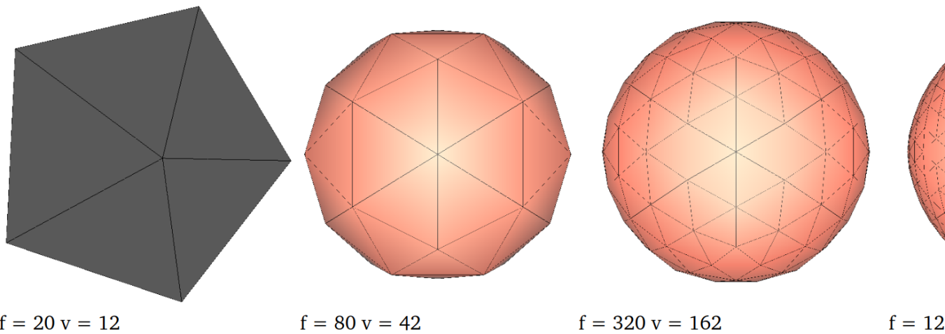
Example: Loop subdivision of Icosahedron
