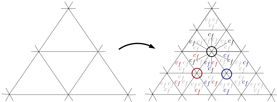
Example: Loop subdivision of Icosahedron
