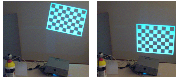
Figure 3. Calibration checkerboard projected from different projectors, one at a time, is viewed by the camera to compute homography with respect to the projector.
