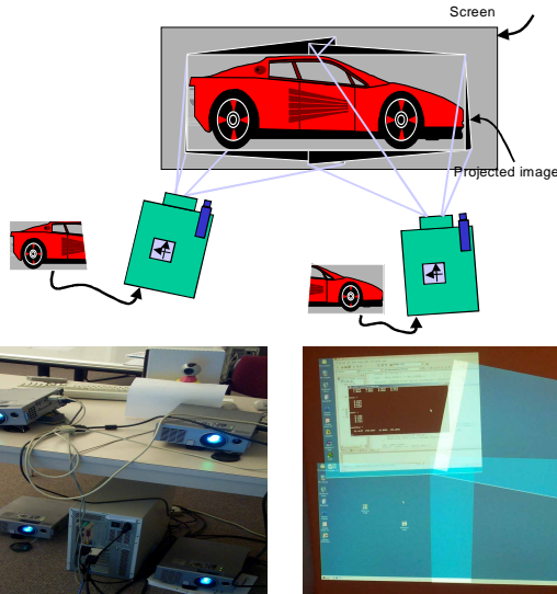
Figure 1. A casually installed projector array. (Top) a schematic diagram (bottom) our four projectors prototype, with viewing camera on the top and resulting projection.
