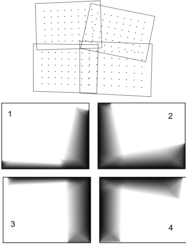
Figure 4. Intensity blending (Top) Projection of illuminated quadrilaterals as recorded in camera coordinates system. The dots indicate points on checkerboard detected for homography computation. (Bottom) The intensity weight for the four projectors. The gray scale indicates the weight in [0,1] . The weights taper off to zero in the overlap region near the projector framebuffer boundary.
